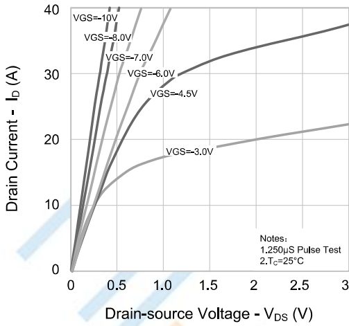
Figure 1. Output Characteristics
