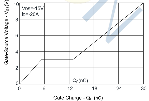
Figure 6. Gate Charge
