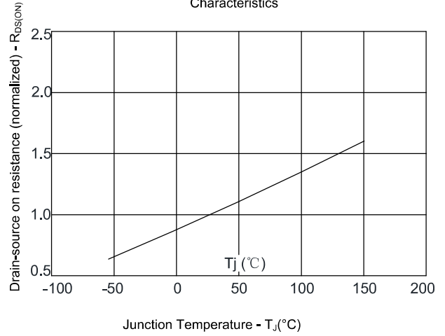
Figure 8. On-resistance vs. Temperature Characteristics
