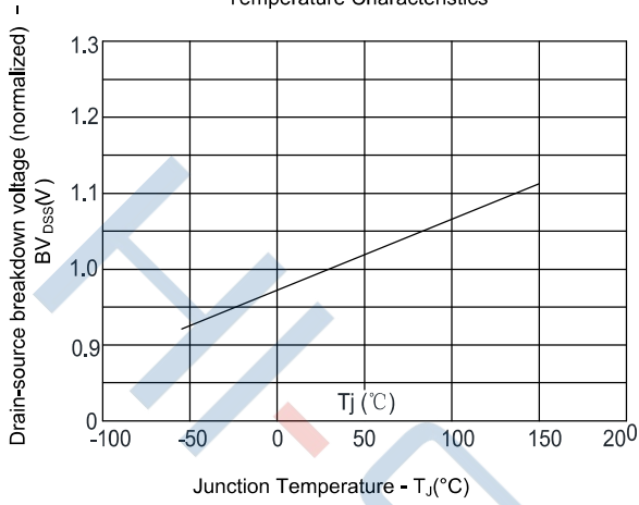
Figure 7. Breakdown Voltage vs. Temperature Characteristics
