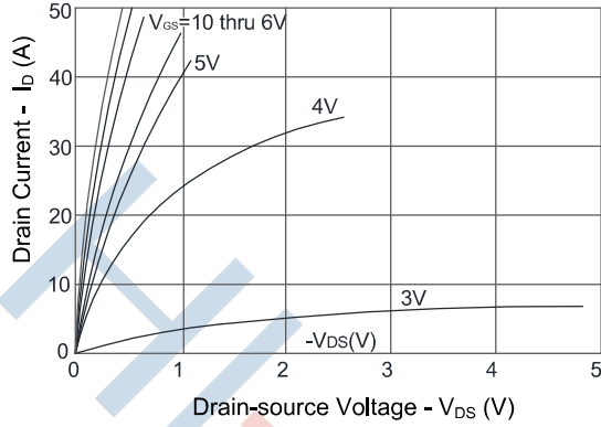
Figure 1. Output Characteristics
